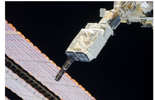
6. NRCSD DEPLOYS CUBESATS
